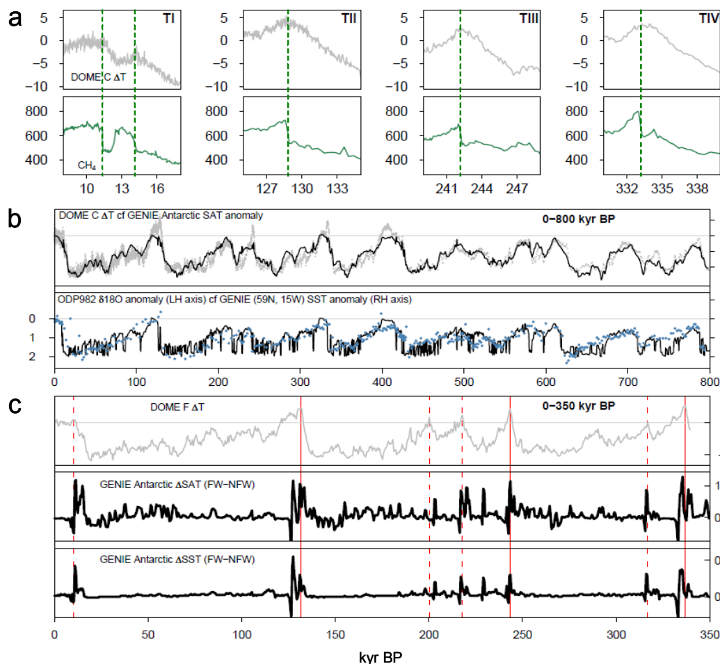
Fig. 1. (a) DOME C \delta D-inferred Antarctic temperature anomaly (Jouzel et al., 2007) (grey) and atmospheric CH 4 concentration (Loulergue et al., 2008) (green) at the last four terminations. (b) 800 kyr records of DOME C Antarctic temperature anomaly (grey) and planktonic \delta^{18}\text{O} anomaly (blue) at ODP site 982 (57.3° N, 15.5° W) (Venz et al., 1999), compared respectively with the GENIE-1 (G FW ) Antarctic SAT anomaly and the SST anomaly at the grid cell centred on 59° N, 15° W. (c) 350 kyr records of DOME F \delta D-inferred Antarctic temperature anomaly (Kawamura et al., 2007) (grey), GENIE-1 meltwater-induced (G FW -G NFW ) Antarctic SAT and SST anomalies. SAT is averaged over Antarctica south of 71° S. SST is averaged over all the Southern Ocean south of 62° S. Note: the simulation in (b) includes meltwater forcing, but the effects in Antarctica (up to \sim 1.5^\circ\text{C} warming) are largely obscured by the larger changes across the terminations.
